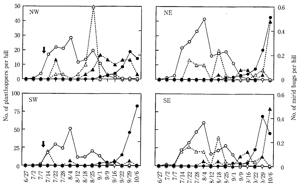
Fig. 2. Seasonal occurrences of rice planthoppers (adults+nymphs) and predacious mirid bugs (adults+nymphs) in 2003 in the paddy field at Chikushino, where Cyrtorhinus lividipennis was released. NW and SW: North and south-western areas of the field ( C. lividipennis release areas), NE and SE: North and south-eastern areas of the field (non-release areas). Arrow: day when C. lividipennis was released. ○: Sogatella furcifera , ●: Nilaparvata lugens , ▲: C. lividipennis , △: Tytthus chinensis . See also legend of Fig. 1.
