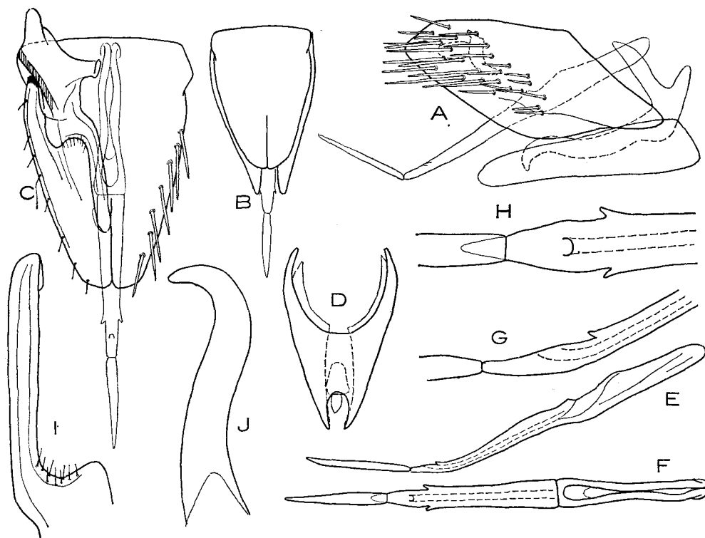
Fig. 5. Peitouellus hokutonis (Mm.) ♂: A—genital [segment, lateral view (45 ×); B—same, ventral view (30 ×); C—pygofer, dorsal view (30 ×); D—genital valve and plates (54 ×); E—aeedeagus and connective, lateral view (54 ×); F—same, dorsal view (54 ×); G—middle part of aedeagus, lateral view (155 ×); H—same, dorsal view (155 ×); I—style, dorsal view (115 ×); J—same, lateral view (115 ×).
