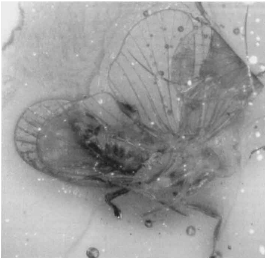
Fig. 13. Bothriobaltia pietrzeniukae gen. and sp. n. Right general view.
