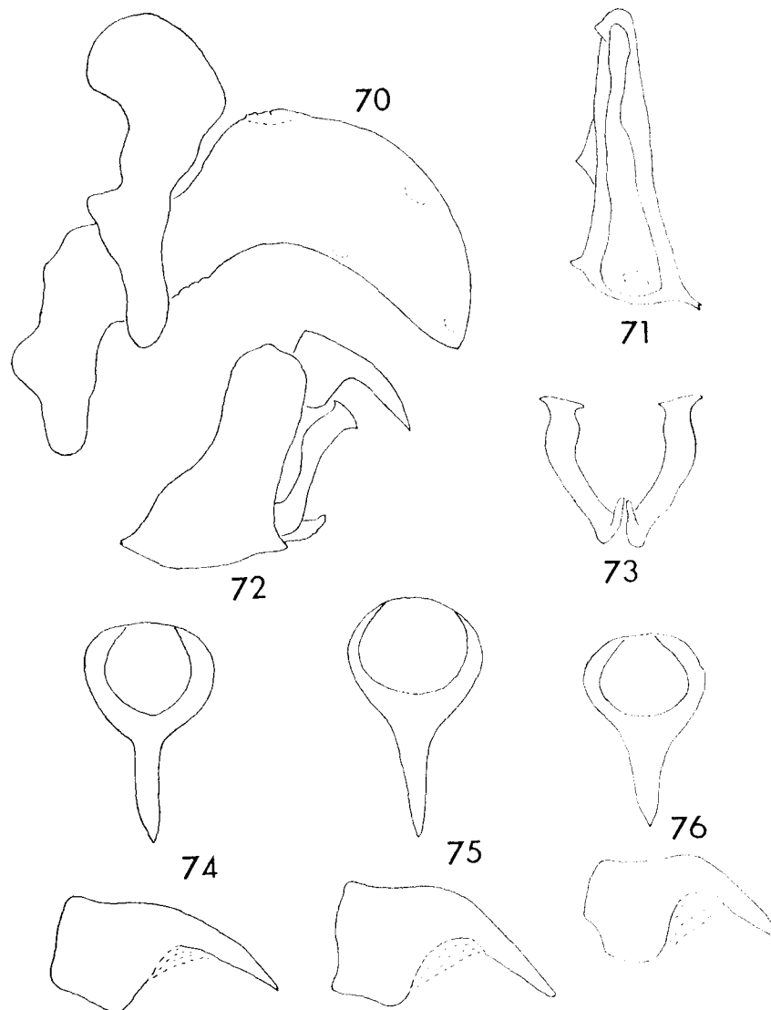
Fig. 70-76, Stobaera azteca . 70, aedeagus in lateral view; 71, aedeagus in dorsal view; 72, male genital capsule in lateral view; 73, styles in posterior view; 74, male anal segment in posterior view above and lateral view below (Veracruz); 75, same (Guerrero); 76, same (San Luis Potosi).
