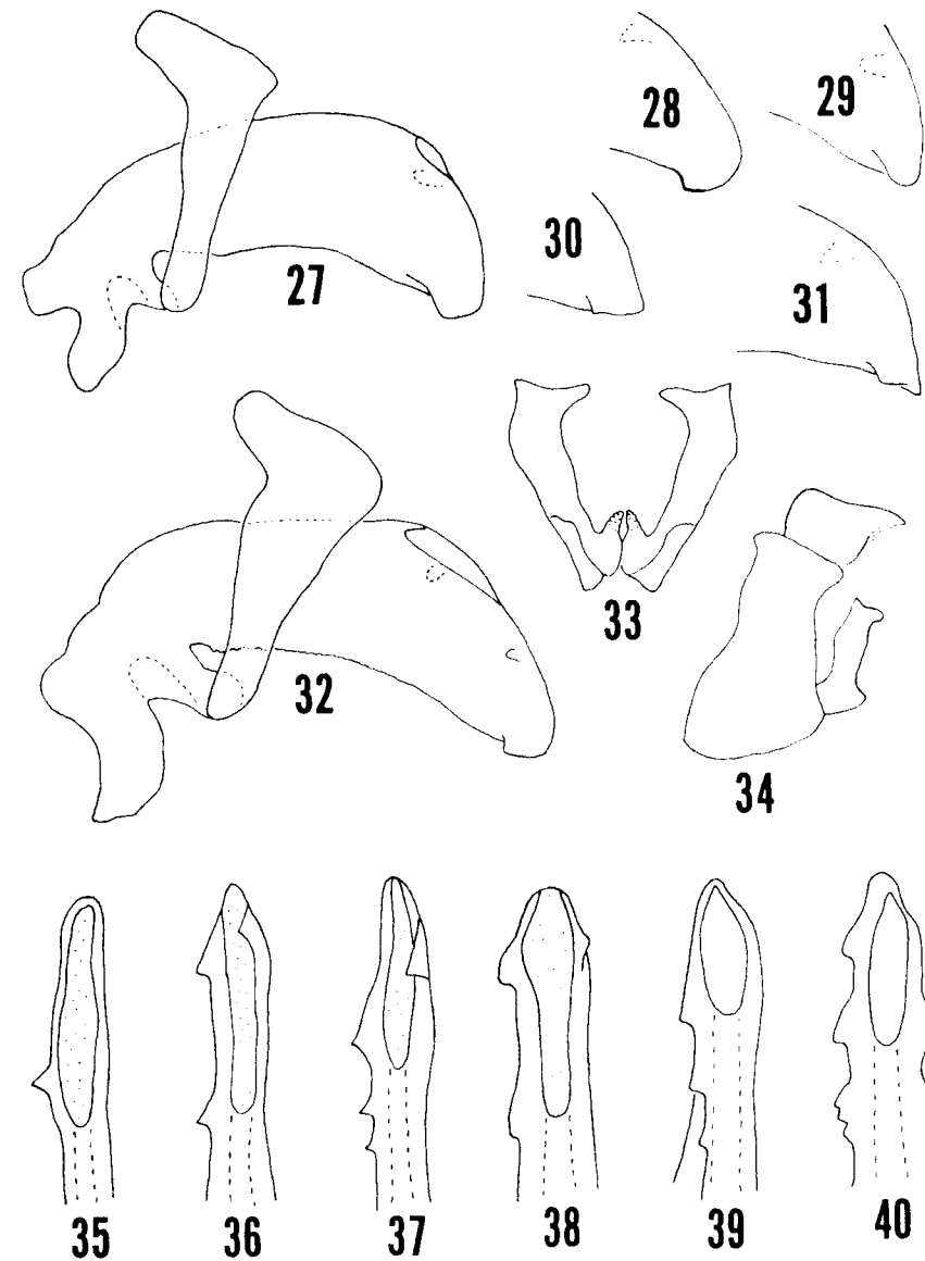
Fig. 27-40, Stobaera concinna . 27, aedeagus in lateral view (Sanford, Fla.); 28, aedeagal apex in lateral view (Superior, Ariz.); 29, same (Sanford, Fla.); 30, same (Brownsville, Tex.); 31, same (Haiti); 32, aedeagus in lateral view (Arcadia, Calif.); 33, styles in posterior view; 34, male genital capsule in lateral view; 35, aedeagal apex in dorsal view (Superior, Ariz.); 36, same (Ariz.); 37, same (Sanford, Fla.); 38, same (Miami, Fla.); 39, same (Fla.); 40, same (Sanford, Fla.).
