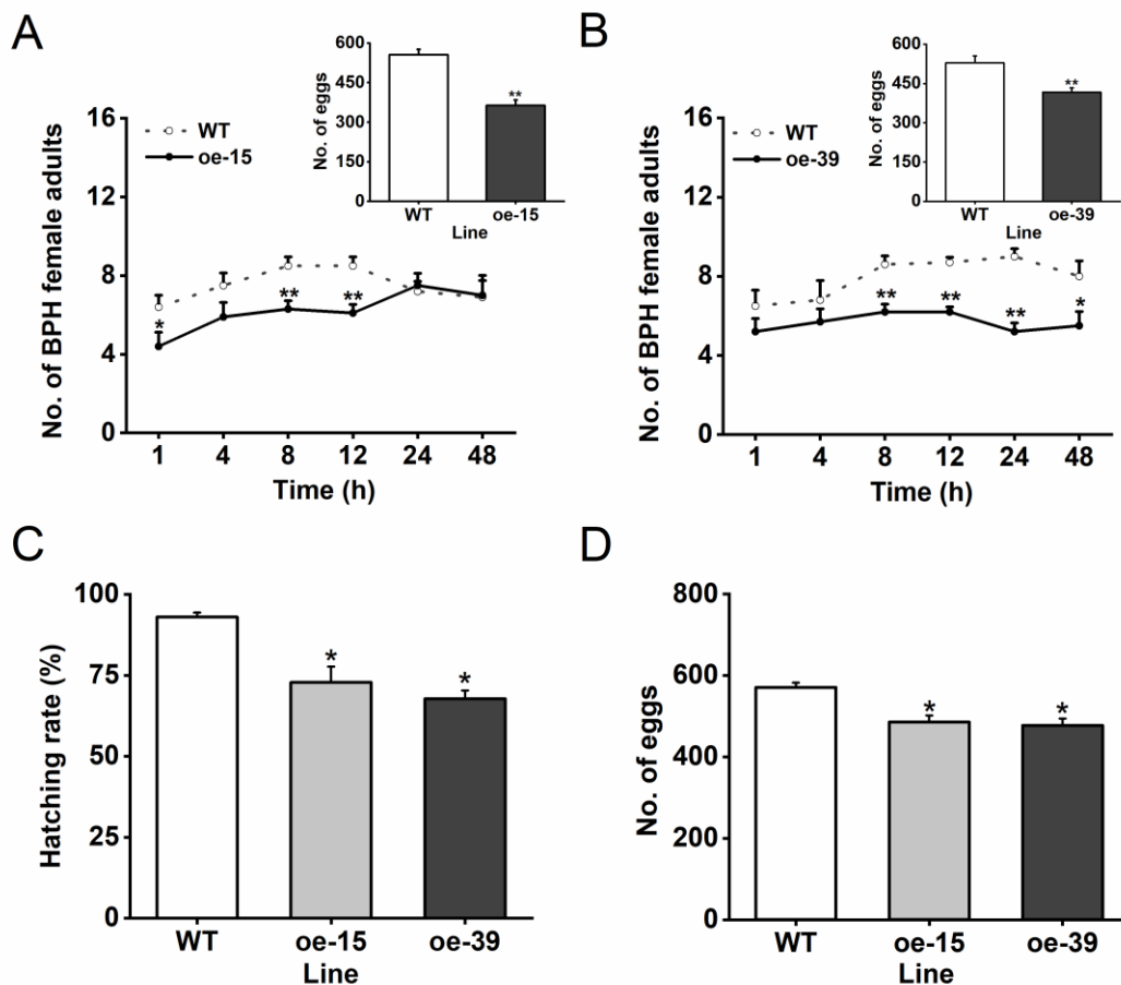
Figure 7. Os6PGDH1 positively regulates rice resistance to BPH. (A,B) Mean number (+SE, n = 10 ) of gravid BPH females per plant on pairs of plants (WT versus oe-15 (A) and oe-39 (B)). Inset: Mean number (+SE, n = 10 ) of eggs per plant on pairs of plants as stated above. Asterisks indicate significant differences between oe6PGDH and WT plants (* p < 0.05 , ** p < 0.01 , Student's t -test). (C) Mean hatching rate (+SE, n = 10 ) of eggs on oe6PGDH plants and WT plants. (D) Mean number (+SE, n = 30 ) of eggs laid by one pair of BPH female and male adults that emerged from oe6PGDH or WT plants. Asterisks indicate significant differences in oe6PGDH lines compared with those in WT plants (one-way ANOVA followed by Duncan's multiple range test, p < 0.05 ).
