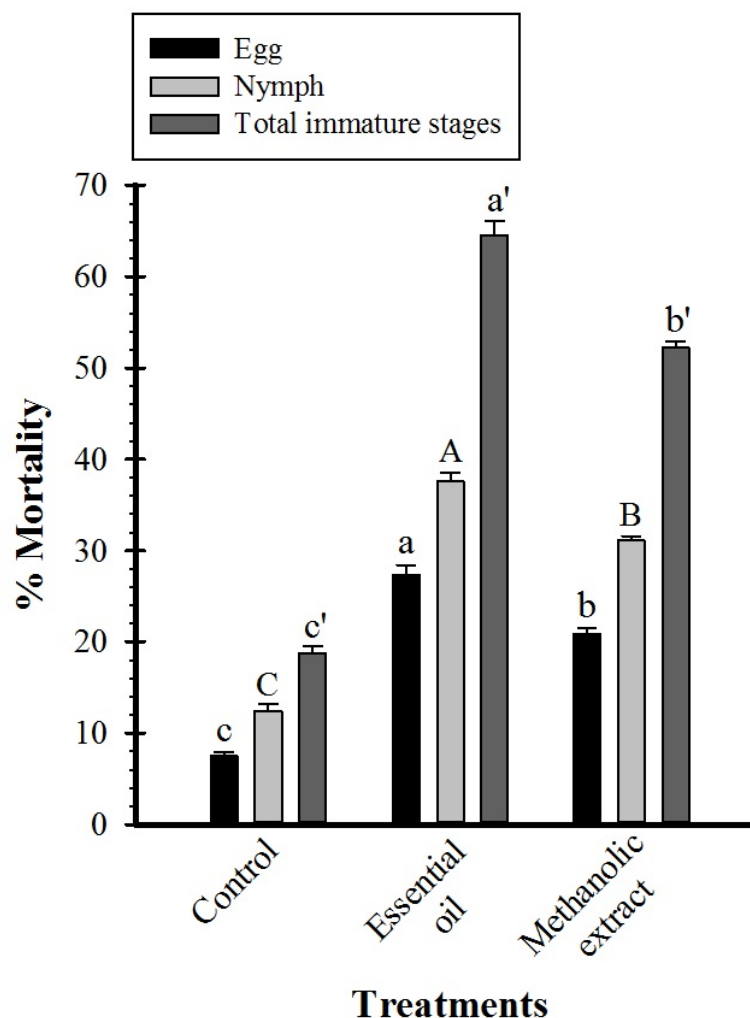
Figure 1. Mean ( \pm SE) percentage mortality of O. lybicus exposed to essential oil and methanolic extract of M. pulegium . The means followed by different letters are significantly different (Tukey test, P < 0.05 ).
