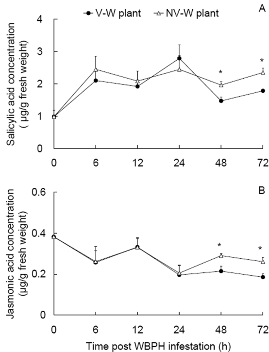
Figure 1. Dynamic concentrations of salicylic acid (A) and jasmonic acid (B) in viruliferous and nonviruliferous WBPH-infested plants (V-W and NV-W plant, respectively) and uninfested plants (0h post WBPH infestation). Values are means \pm SE. * indicates significant differences between the viruliferous and nonviruliferous WBPH-infested plants at a certain time point post WBPH infestation (independent sample t -test, P < 0.05 ).
