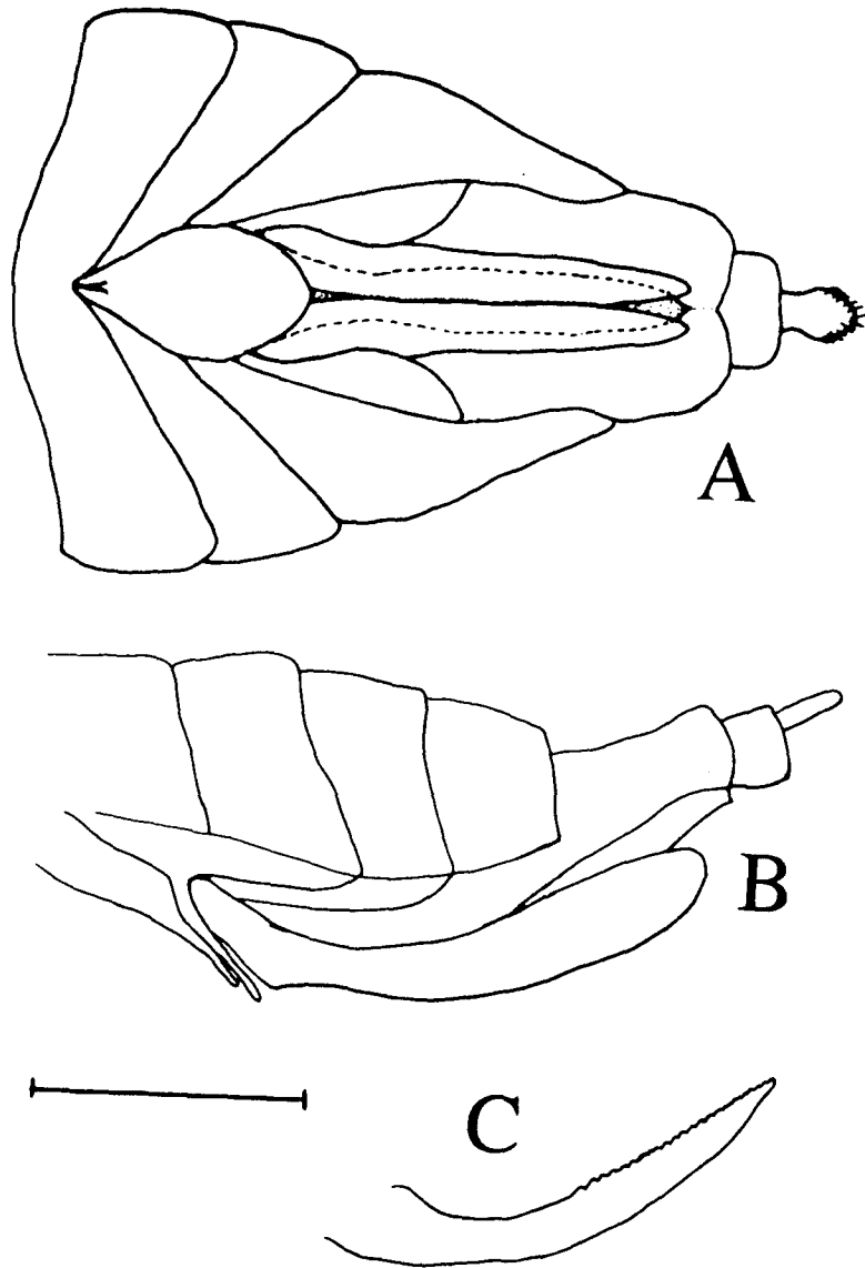
Fig. 2. P. spinata female genitalia. (A) Ventral view. (B) Lateral view. (C) Lateral view of ovipositor (median gonapophyses of segment 9). Bar = 0.5 mm.
