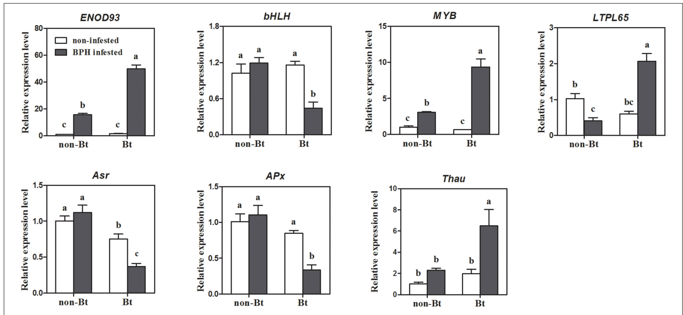
FIGURE 2 | Quantitative RT-PCR verification of seven genes likely involved in the variation of BPH performance on Bt rice. ENOD93 , early nodulin 93 (LOC_Os06g04990); bHLH , Helix-loop-helix DNA-binding domain containing protein (LOC_Os01g38610); MYB , myb-like DNA-binding domain, SHAQKYF class family protein (LOC_Os04g56990); LTP65 , protease inhibitor/seed storage/LTP family protein (LOC_Os01g59870); Asr , aba stress-ripening (LOC_Os01g73250); APx , L-ascorbate oxidase (LOC_Os06g37150); Thau , thaumatin-like protein (LOC_Os12g43440). Error bars represent SD values ( n = 3 ); different letters indicate significant differences ( P < 0.05 ).
