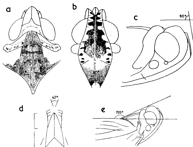
FIG. 8. Alticeps vigilis sp. nov. (a) vertex, pronotum and mesonotum; (b) frons and clypeus; (c) head and thorax in profile; (d) vertex viewed at right angles to disc; (e) body profile showing raised posture of head and thorax.
